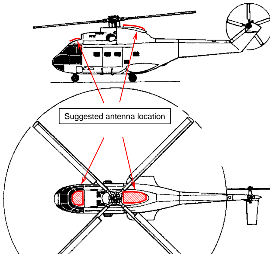
Figure 1. Suggested location of Indigo antenna
