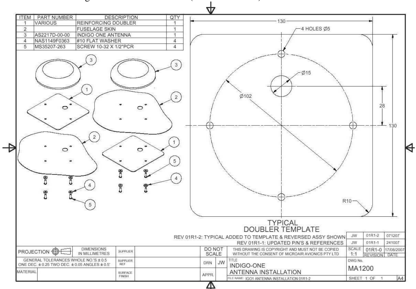
Figure 3. Doubler details.
