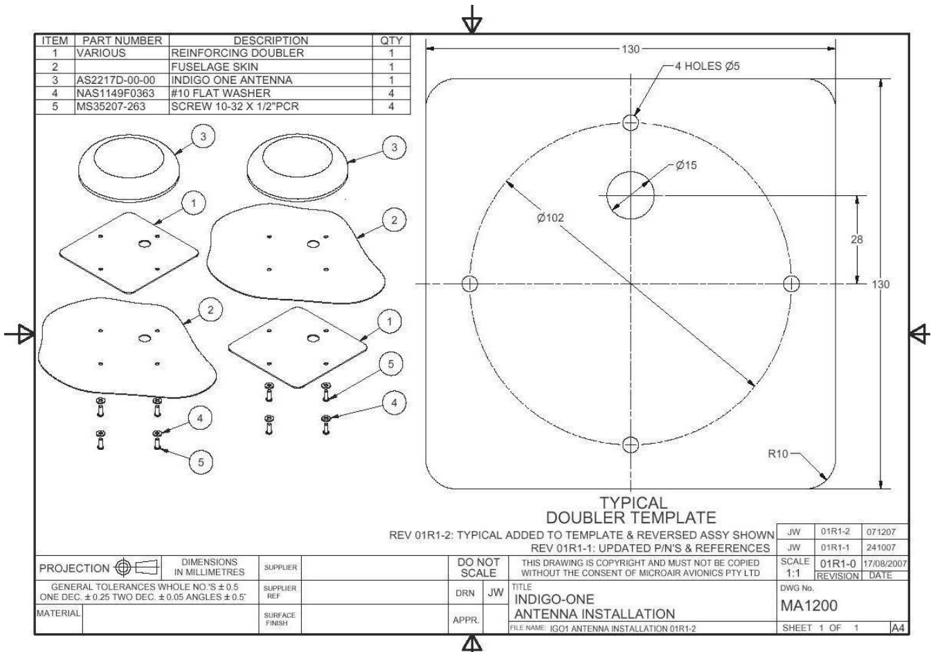
Figure 3. Doubler details.
