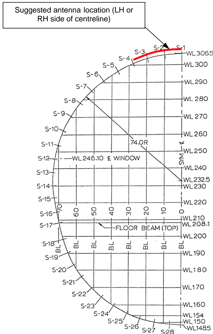
Figure 2. Suggested location of Indigo antenna Boeing 737 series
