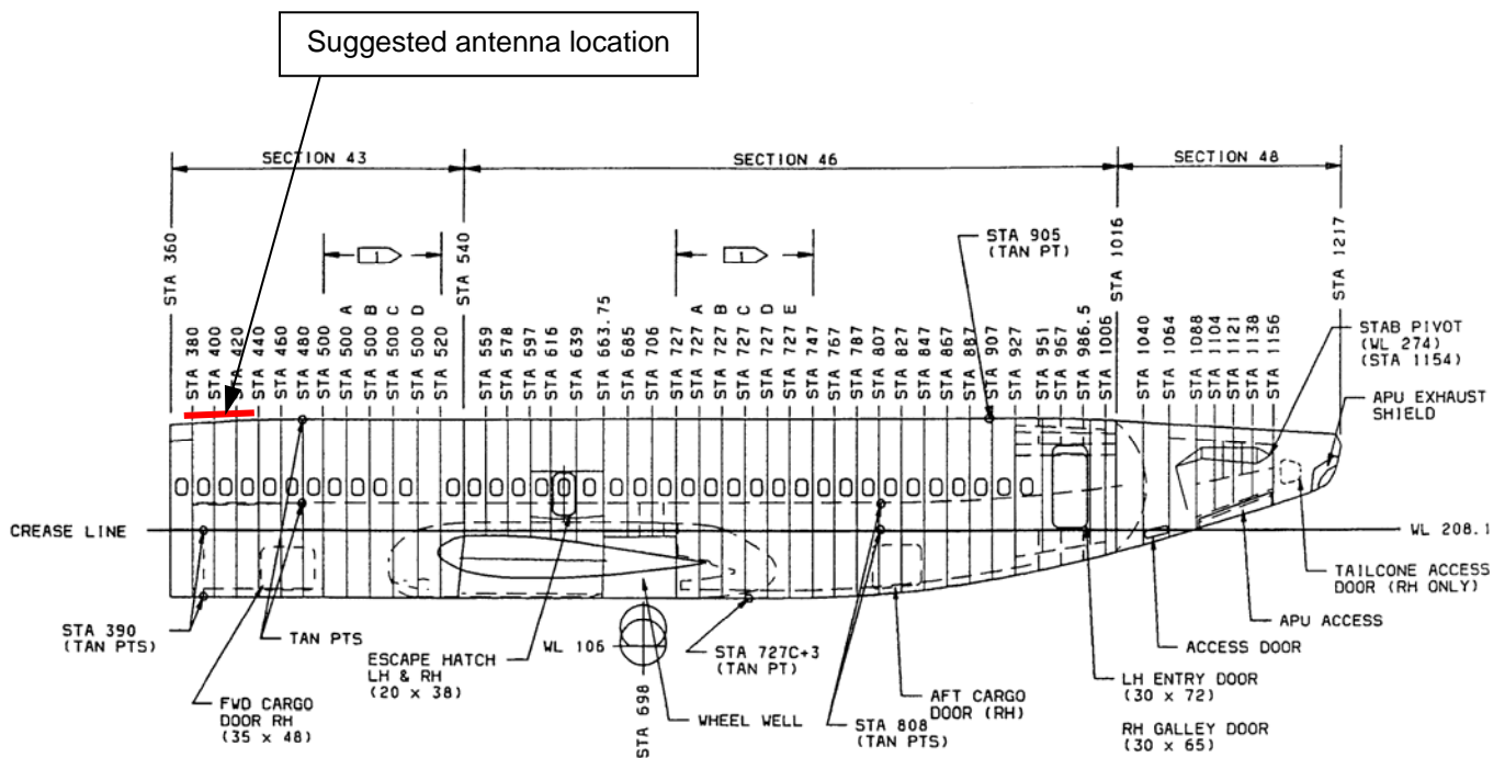
Figure 1. Suggested location of Indigo antenna Boeing 737 series
