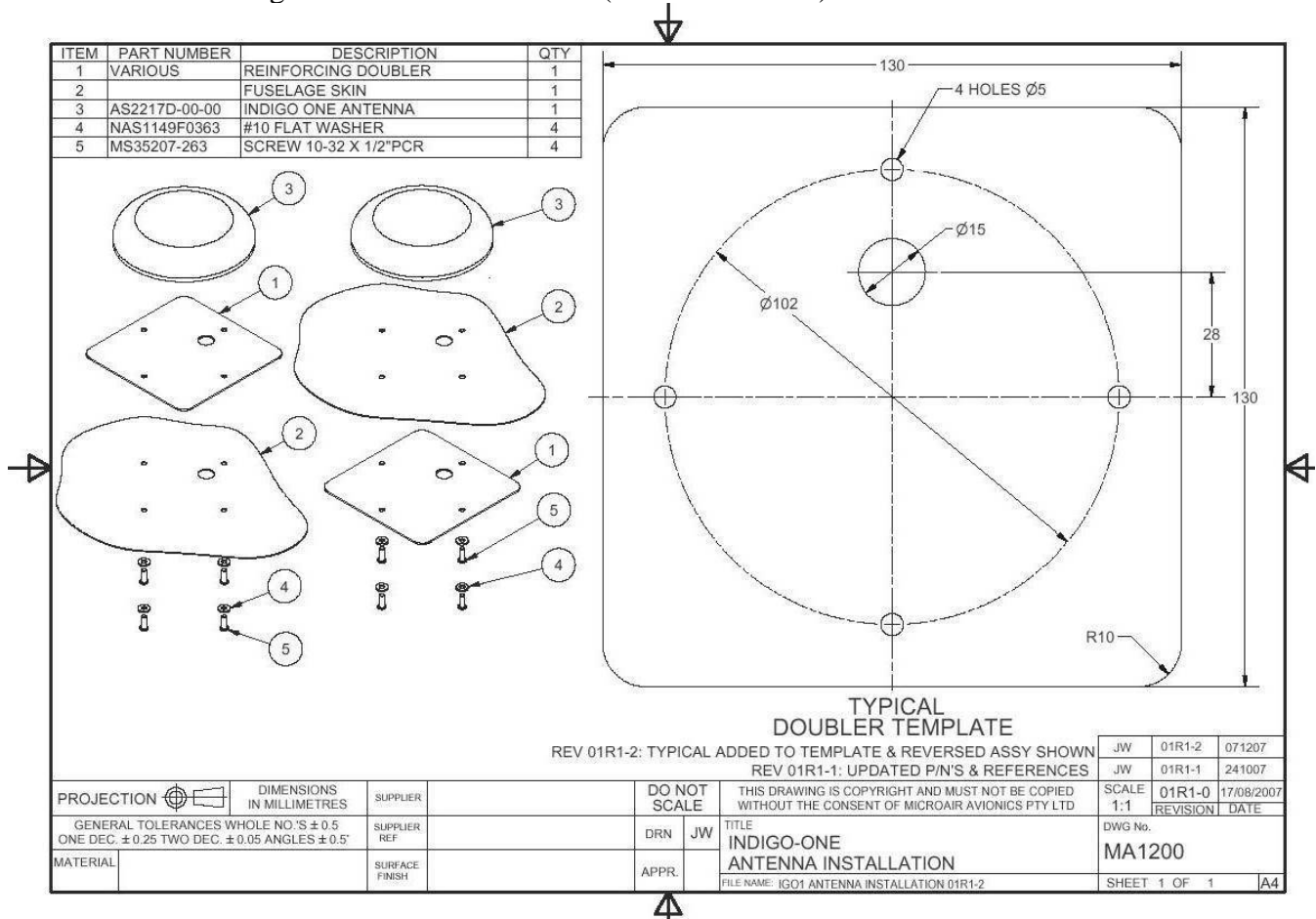
Figure 3. Doubler details.
