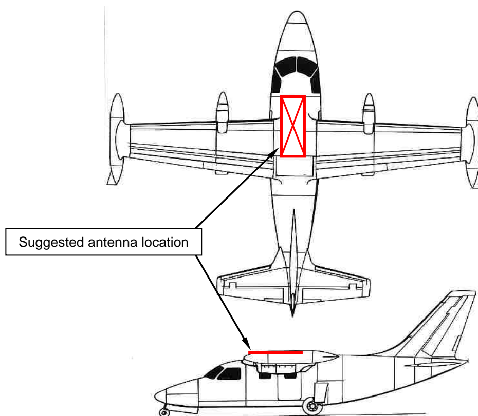
Figure 1. Suggested location of Indigo antenna
